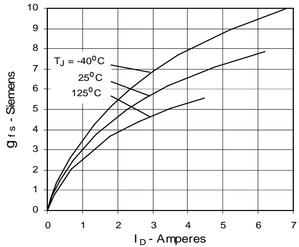
Fig. 8. Transconductance
